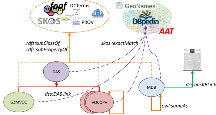
Fig. 1. The Dutch Ships and Sailors Linked Data cloud. The individual datasets are represented by ovals in the bottom half of the image. Internal links are represented by arrows. External links are represented by dotted arrows.
